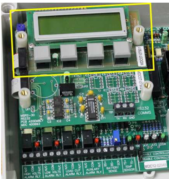
The MSR2-30 Display PCB Assembly (outlined in yellow) fitted to an MSR2-30 Control PCB
