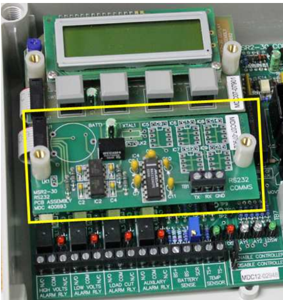
The MSR2-30 RS232 Interface PCB Assembly (outlined in yellow) fitted to an MSR2-30 Control PCB
