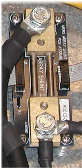
PN 400790 in a typical installation.
