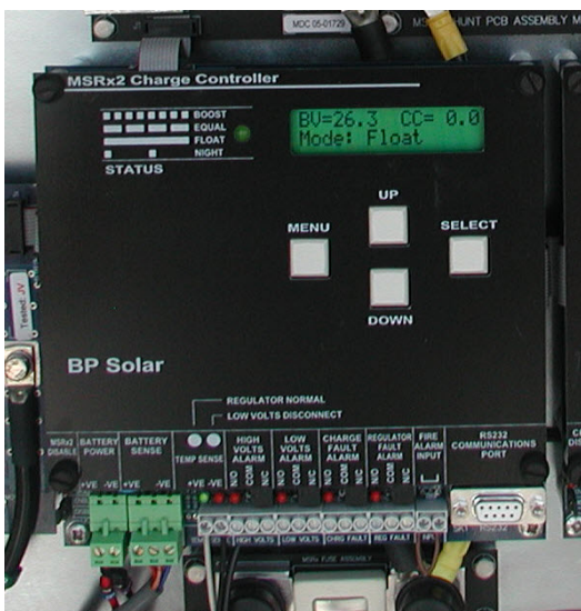
PCB Assembly 400848 installed in controller PN 101103
