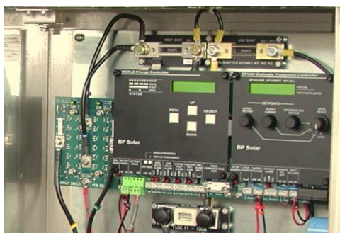
Typical installation of PN 400849 (shown on right including fascia panel).
