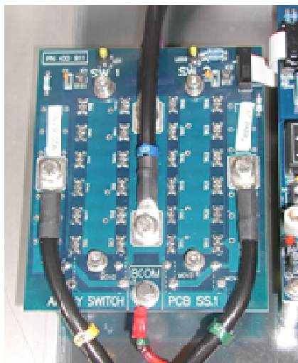
Assembly 400911 fitted to mounting plate.
