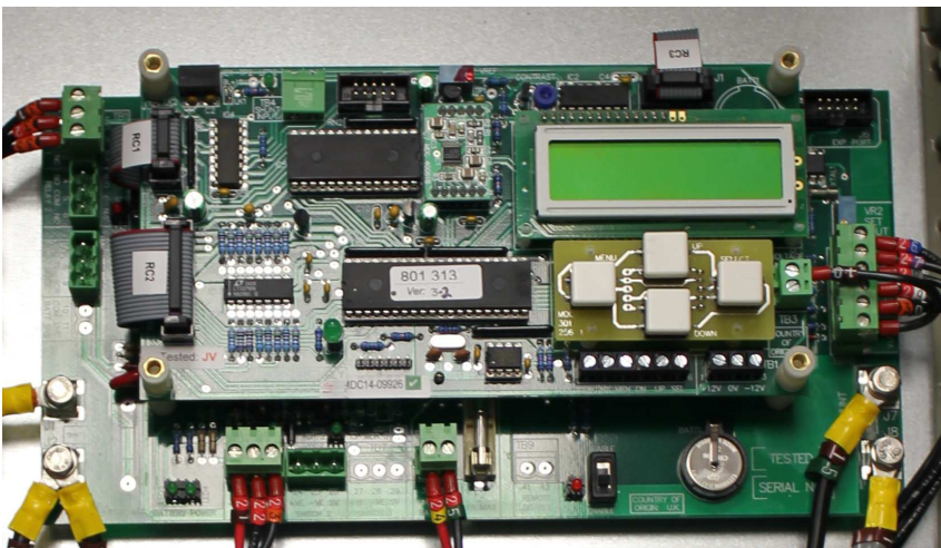
PCB assembly 401954-2 shown on left (fitted below Control PCB assembly 401764)
