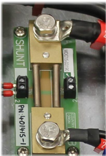
PN 401415 in a typical installation
